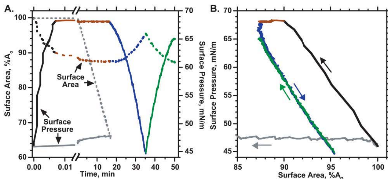
FIGURE 1 Transformation of POPC monolayers by rapid compression. Films spread to initial surface pressures <42 mN/m were compressed at 26^{\circ}\text{C} and 0.005\text{ min}^{-1} to 46 mN/m, just below \pi_c . The bubble was then manipulated by infusion of buffer at a constant rate of either 1.4\% initial volume/min (gray lines; initial area compression of 0.01\text{ min}^{-1} ) for 17 min, or 109\% initial volume/s (black lines; area compression of 23.1\text{ min}^{-1} ) until surface pressure reached 68 mN/m. Surface pressure of the rapidly compressed film was held constant for 15 min (red lines), after which it was expanded to lower surface pressure at 2.5\% initial volume/min (blue lines), and then recompressed at the same rate (green lines). (A) Variation of surface pressure (solid lines, right axis) and area (dashed lines, left axis) with time. Surface area is expressed relative to the initial area at 46 mN/m ( A_0 ). Split timescale shows that the more rapid compression lasted \sim 0.4 seconds. (B) The same measurements plotted as surface pressure versus surface area.
