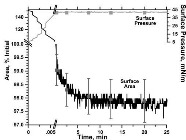
FIGURE 3 Relaxation after a rapid change in surface pressure below \pi_c . Films of POPC spread to 5 \pm 4 mN/m were compressed at 74 \pm 6 min ^{-1} to 41 \pm 1 mN/m and then held at constant surface pressures. Area is expressed relative to the initial value when the film first reached its isobaric surface pressure. The split time and area scales distinguish the initial rapid compression from the subsequent isobaric relaxation. The curve shown is representative of four experiments. Symbols indicate mean \pm SD at selected times.
