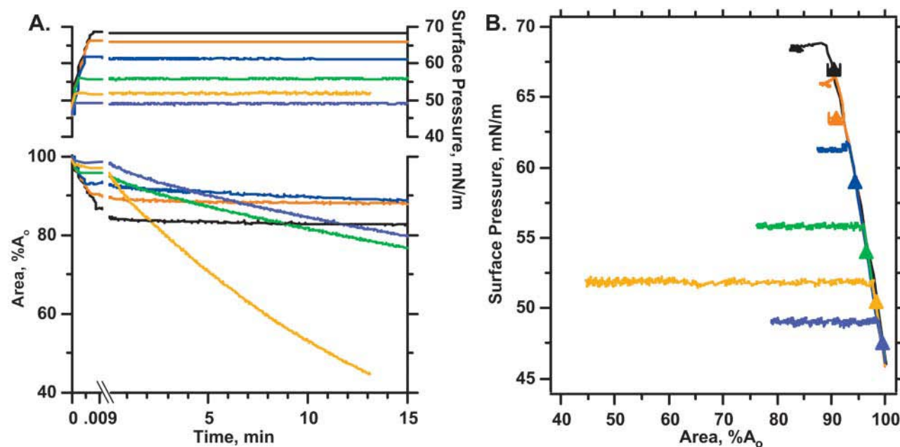
FIGURE 4 Rapid initial compression followed immediately by isobaric compression. Monolayers of POPC spread to <42 mN/m were first compressed at 26^\circ\text{C} and <0.005 min ^{-1} to 46 mN/m and then at 23 \pm 5 min ^{-1} to different target surface pressures. Isobaric compression then maintained the final surface pressure achieved at the end of the rapid compression. Experiments lasted at least 15 min or until hydrostatic pressure exceeded the limits of the apparatus (3.5 atm). (A) Variation of surface area (lower left axis) and surface pressure (upper right axis) with time. Area is normalized to the initial value at 46 mN/m ( A_0 ). (B) Surface pressure-surface area isotherms. Curves of the same color in Fig. 4, A and B, indicate presentations of the same data. For purposes of clarity, results are presented for individual experiments. Symbols in Fig. 4 B give mean area \pm SD at specific surface pressures during the rapid compression for at least five experiments in each case. Error bars that are not evident are less than the size of the symbols. Error of the measurements during the isobaric compressions is given in Fig. 5.
