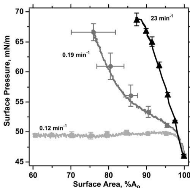
FIGURE 2 Compression at different rates. Monolayers of POPC spread to surface pressures <42 mN/m were first compressed at 26^{\circ}\text{C} and 0.03\text{ min}^{-1} to 46 mN/m, and then to higher surface pressures at the indicated rates of area-compression expressed as d(\ln A)/dt (see Methods). Area is normalized relative to the initial area at 46 mN/m ( A_0 ). Curves give data from representative experiments. Symbols give mean \pm SD at selected points averaged at common volumes for both area and surface pressures in three experiments.
